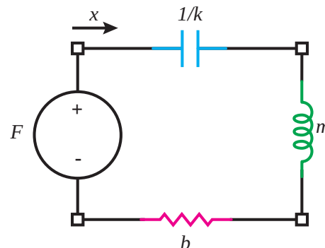
Equivalent circuit
