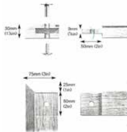
Fig. 27.2 Joint details
